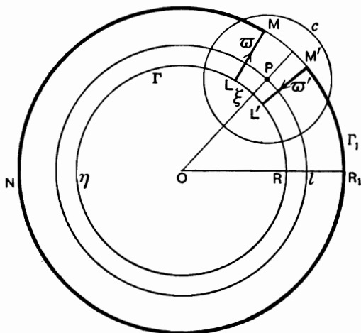
The contribution of \Sigma j^1_{p,q} .
